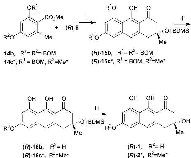
Scheme 5 Reagents and conditions: i, LDA, 14 , THF, -78^{\circ}\text{C} , then ( R )- 9 ; ii, H 2 , Pd/C; iii, HF, CH 3 CN; * = 13 C label.
